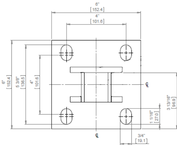
Concrete anchor plate
