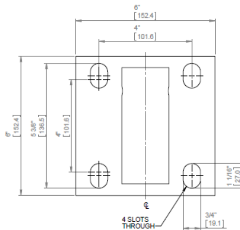
Chute/Crush mounting plate
